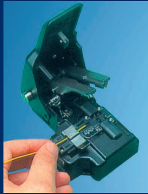
Fibre Placing
